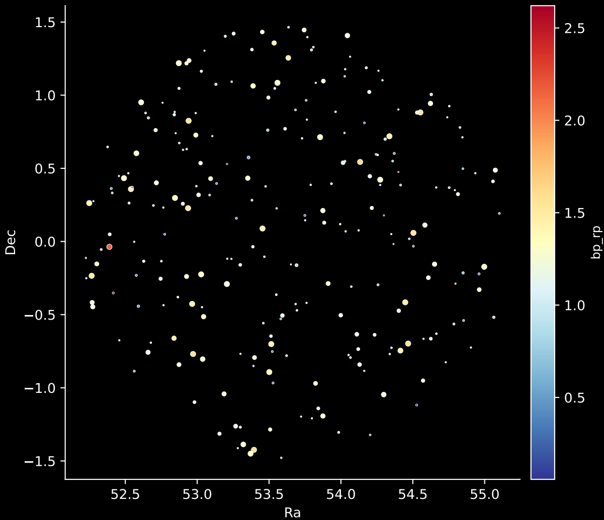
APOGEE DR17 Field: [048-27_MGA] Stars: 248
