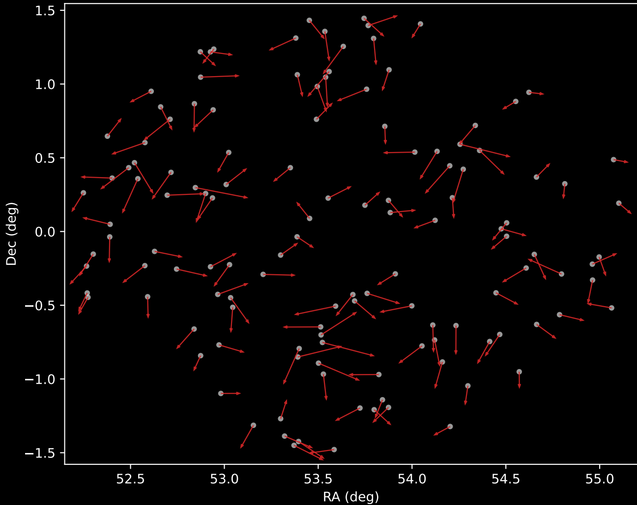
APOGEE DR17 Cluster 6 Proper Motion Vectors (n=129)
