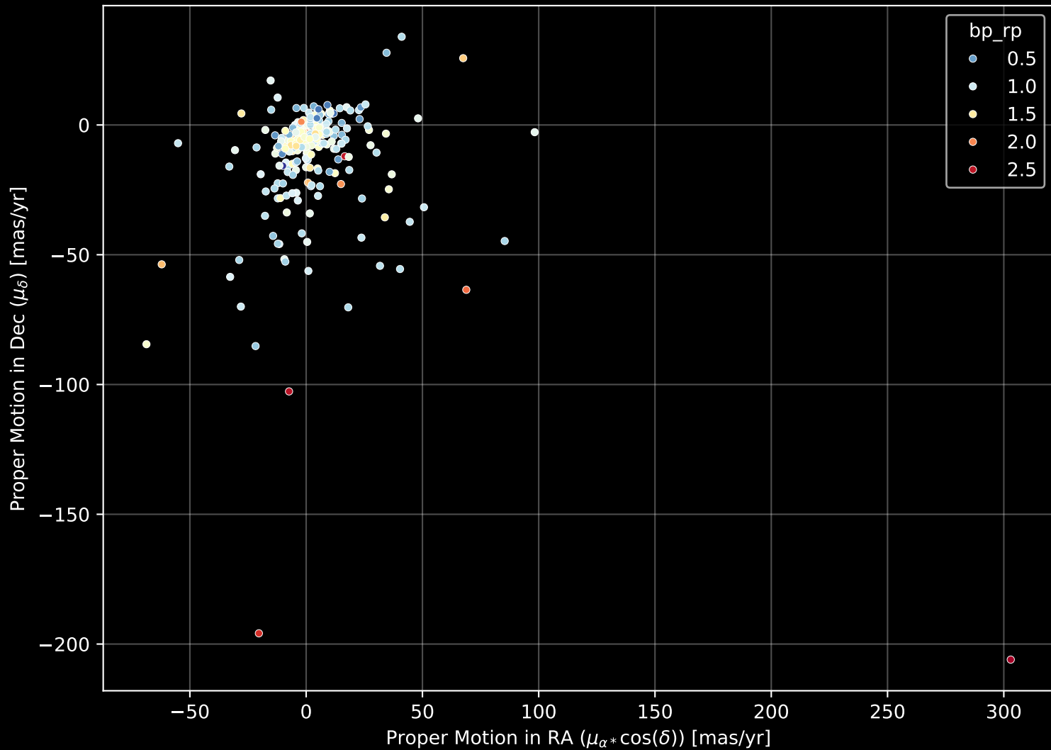
APOGEE DR17 Field: [048-27_MGA] Proper Motion Diagram (n= 248)
