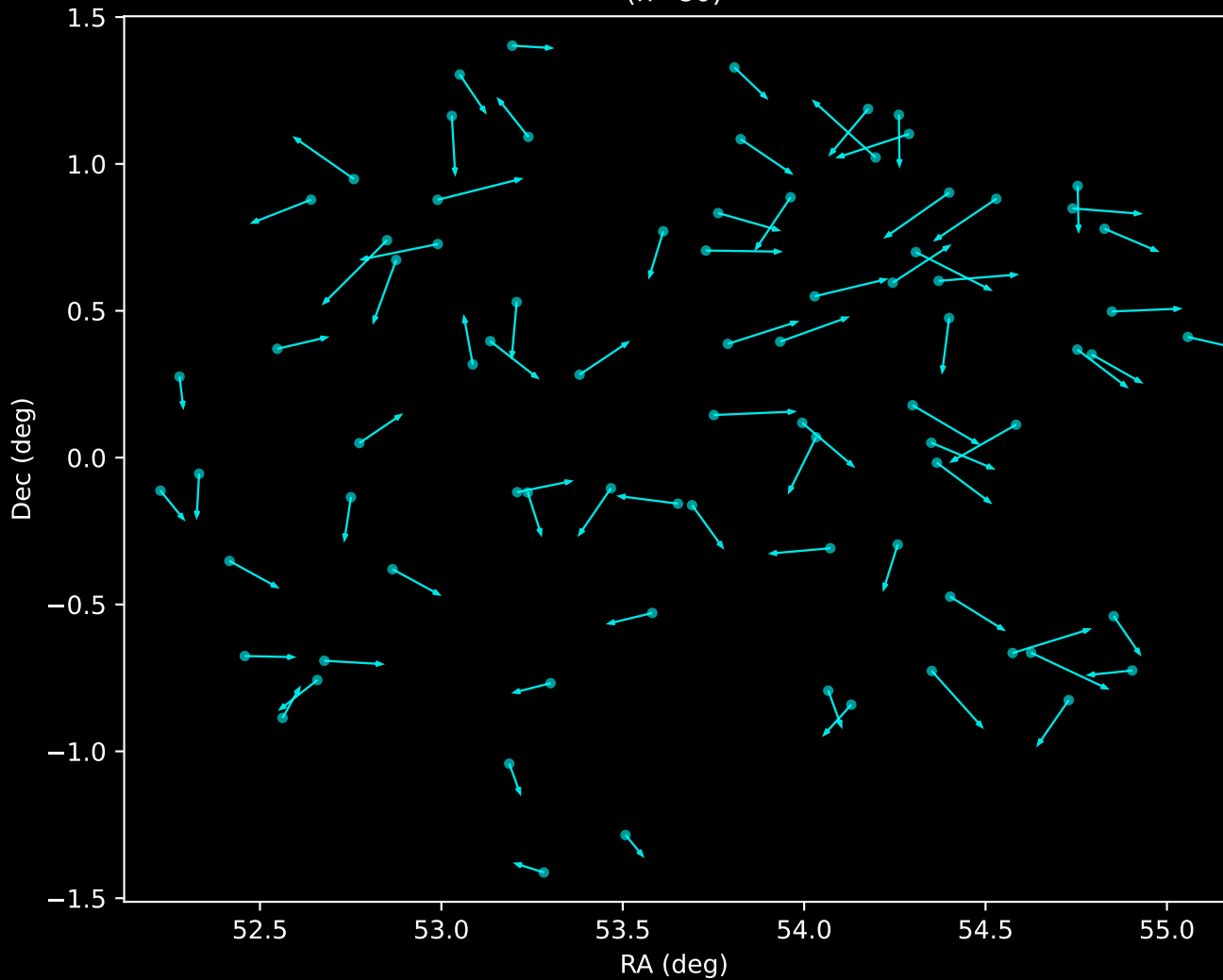
APOGEE DR17 Noise Stream Proper Motion Vectors (n=80)
