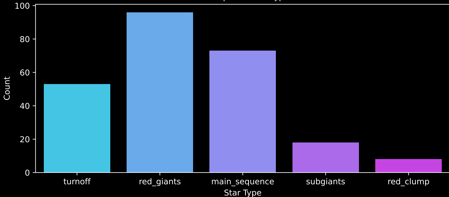
APOGEE DR17 Field: [048-27_MGA] Count plot of Star Type
